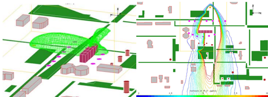
Figure 7. Dispersion plume in isometric view (left) and on a horizontal plane on the ground (right)
