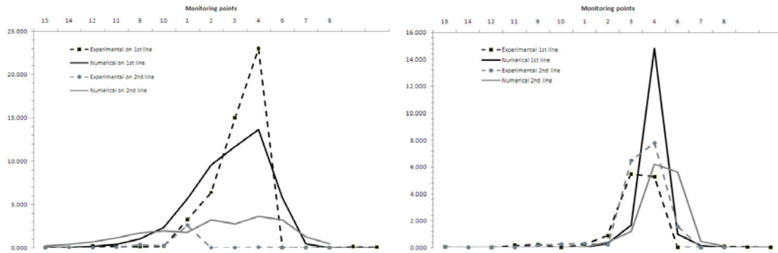
Figure 2. Comparison of measured and simulations concentrations for the 1 st and 2 nd line of sensors at 13:30 (left) and 13:40 (right)
