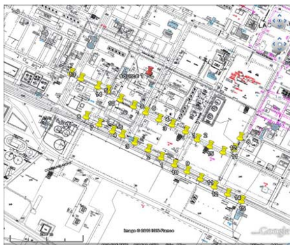
Figure 2. Location of source (red) and sensors (yellow) for test case 1
