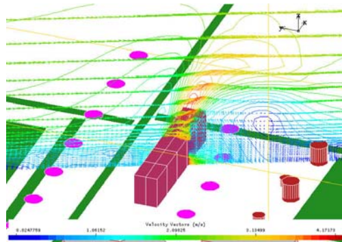
Figure 5. Velocity vectors on a section through the cooling towers
