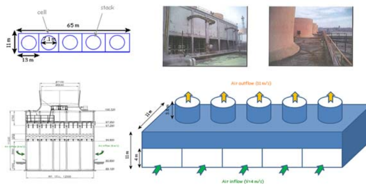
Figure 4. Details of the cooling towers
