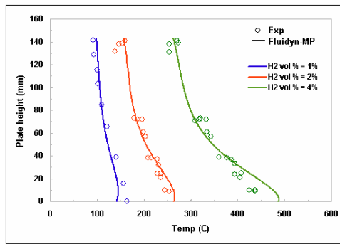
Fig. 10: Catalytic plate temperature profile with different concentrations of H_2
