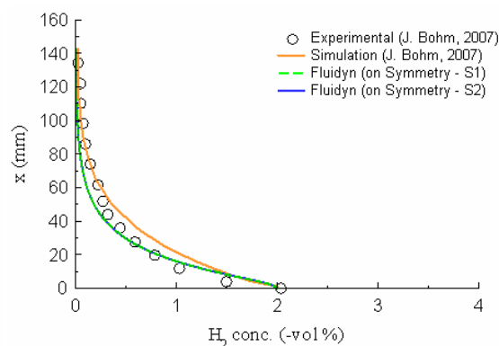
Fig. 7: Hydrogen concentration profile
