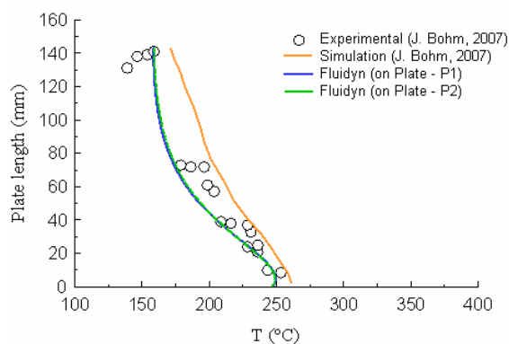
Figure 6: Catalytic plate temperature profile
