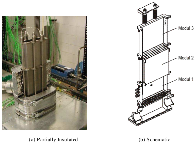
Fig. 2: REKO-3 Test facility
