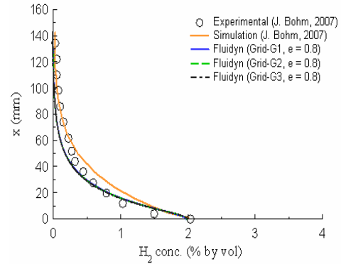
Fig. 5: Hydrogen concentration profiles
