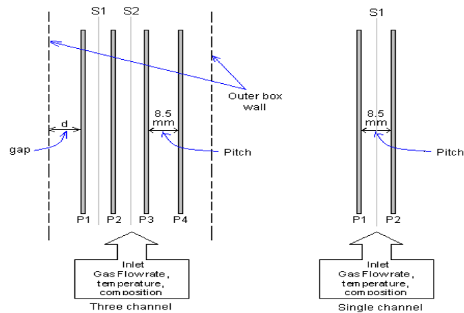
Fig. 3: Geometry for three channel and single channel cases
