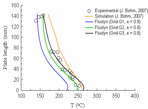
Fig. 4: Catalytic plate temperature
