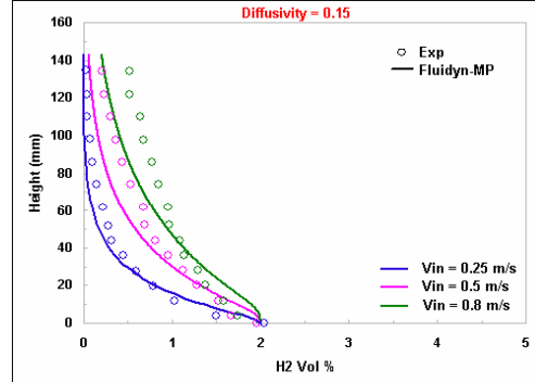
Fig. 13: Concentration profile for different flow rates
