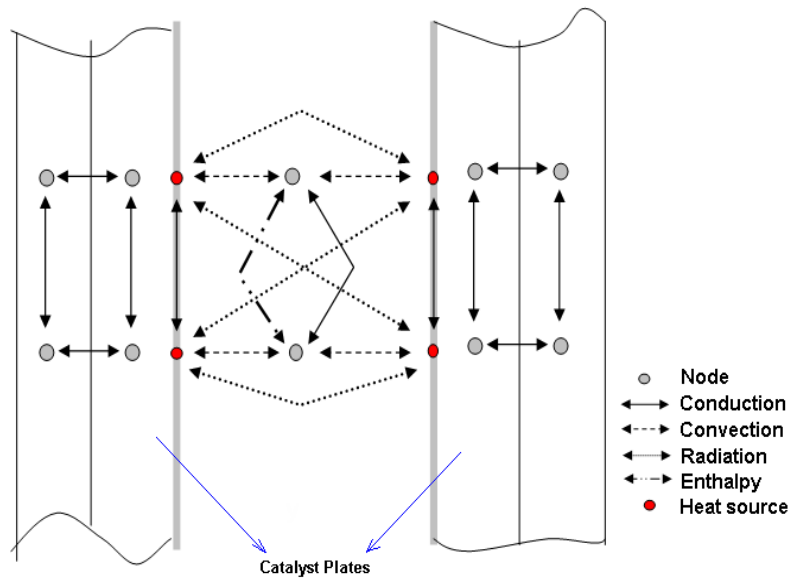
Fig. 1: Modes of Heat transfer in the recombiner model
