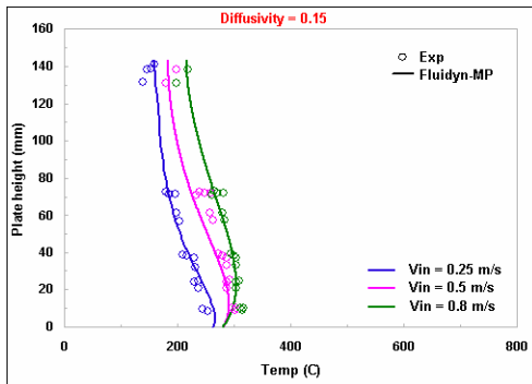
Fig. 12: Catalytic plate temperature profile for different flow rates
