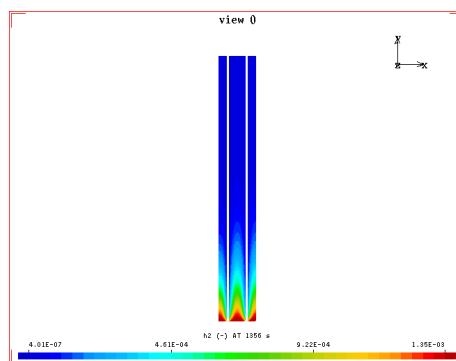
Fig. 9: Contour plot for H_2 concentration
