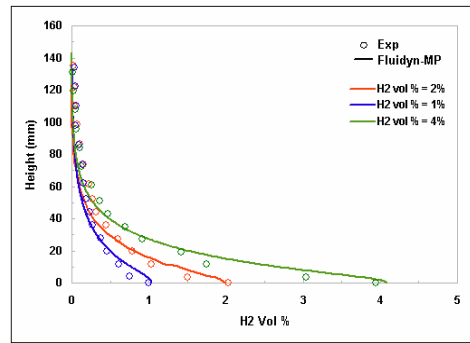
Fig. 11: Hydrogen concentration profile with different concentrations of H_2
